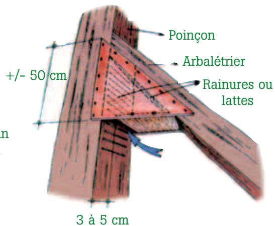
Construction sur angle poinçon-arbalétrier
